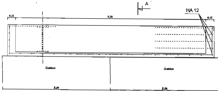
DETAIL A (ferrailage)
